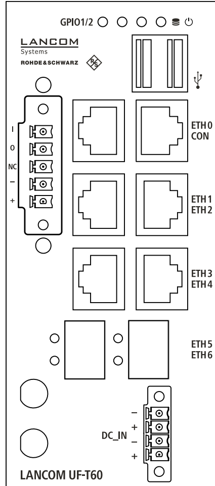
LANCOM R&S®Unified Firewall UF-T60
