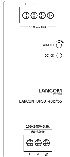
LANCOM DPSU-480/55 (NEW)
